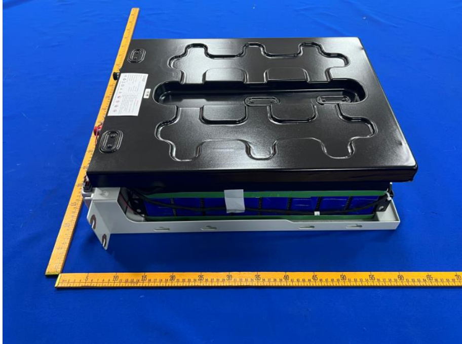
样品图片,内部电池模块 (Sample photograph, internal battery module) -16
