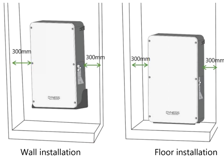
Figure 3-3 Mounting Space Requirements Table 3-1 Installation Steps
